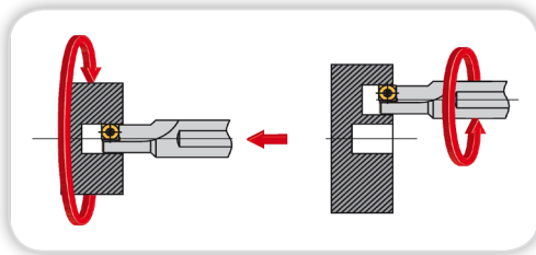
Drilling with flat bottom
